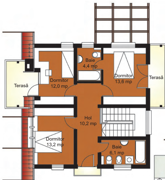
PLAN MANSARDĂ
